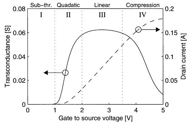
Fig. 6. Typical LDMOS transconductance g_m and drain current I_{ds} with different operating regions indicated.
